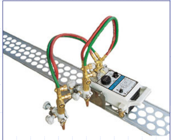
HK-12 (II) Double Torch
